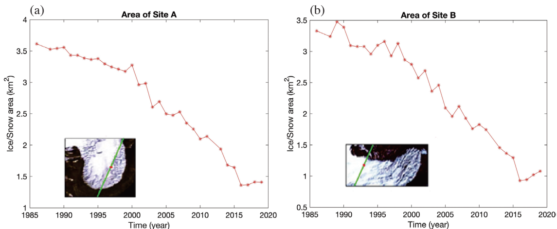
Fig. 12. Glacier area changes from Landsat imagery around (a) site A, and (b) site B. Inserted are sample Landsat glacier images (in white) and the ground track of T/P pass 155.
