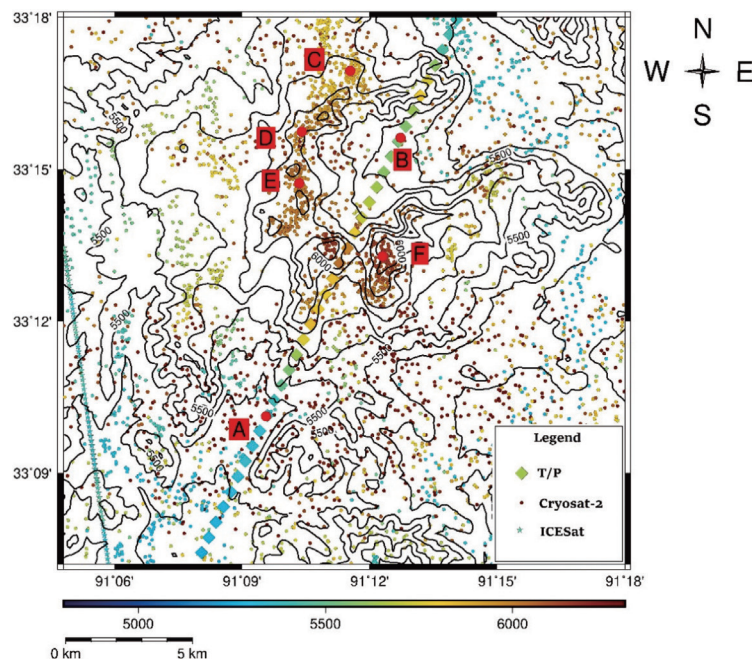
Fig. 3. Elevations (in meter) over part of Tanggula Mountains from the T/P-Jason, Cryosat-2, and ICESat altimeters. A-F are sites for Cryosat-2 determination of glacier elevation change (sites A and B are along T/P pass 155).
