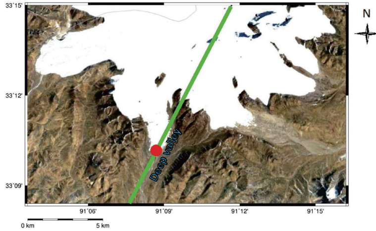
Fig. 10. A 2016 image (selected from all the 1984–2016 Google Earth images) shows that site A (red dot) is over a deep valley, where glaciers near the T/P ground track (in green) was close to disappearing in 2016.
