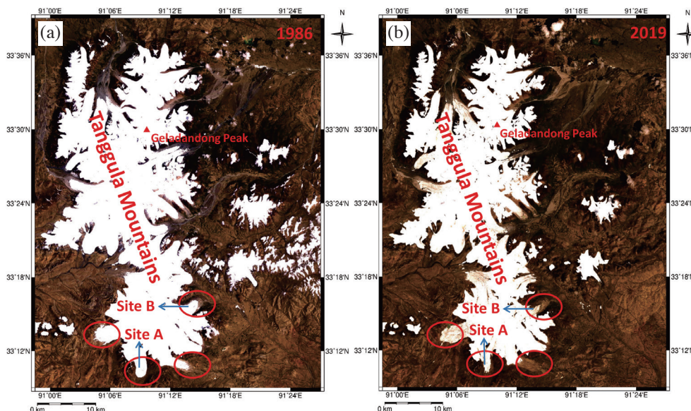
Fig. 1. Two sample Landsat images over Tanggula Mountains. (a) Landsat-5 image on 30 July 1986 and (b) Landsat-8 image on 25 July 2019. These two images show reductions of glacier areas near sites A and B (see Figs. 2c and d) and other glacier terminuses between 1986 and 2019.
