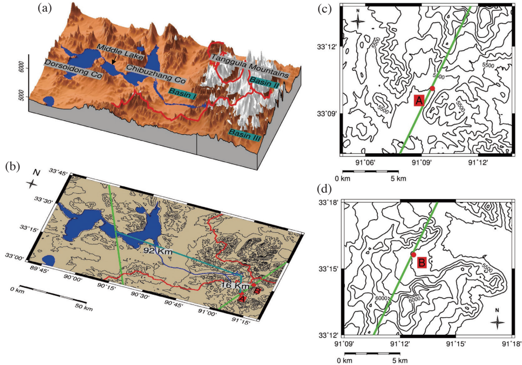
Fig. 2. (a) The topography over Tanggula Mountains, Chibuzhang Co and its sister lake Dorsoidong Co. The Middle lake is part of Chibuzhang Co and the two lakes have the same level. The glaciers, shaded in white, are defined by the Global Land Ice Measurements from Space (GLIMS) database ( https://www.glims.org ). The lakes (blue-shaded) are based on the GSHHG database. (b) The ground tracks of T/P pass 155 (over sites A and B) and 242 (over Chibuzhang Co). The red points show sites A and B in Table 1. (c) The elevation contours and T/P pass 155 at site A, and (d) site B. The red polygons represent three catchment basins around Tanggula Mountains. Basin I supplies source water to Chibuzhang Co, Basin II to the Yangtze River, and Basin III to Selin Co in Tibet (at about 31.81°N, 89.01°E, not in this figure).
