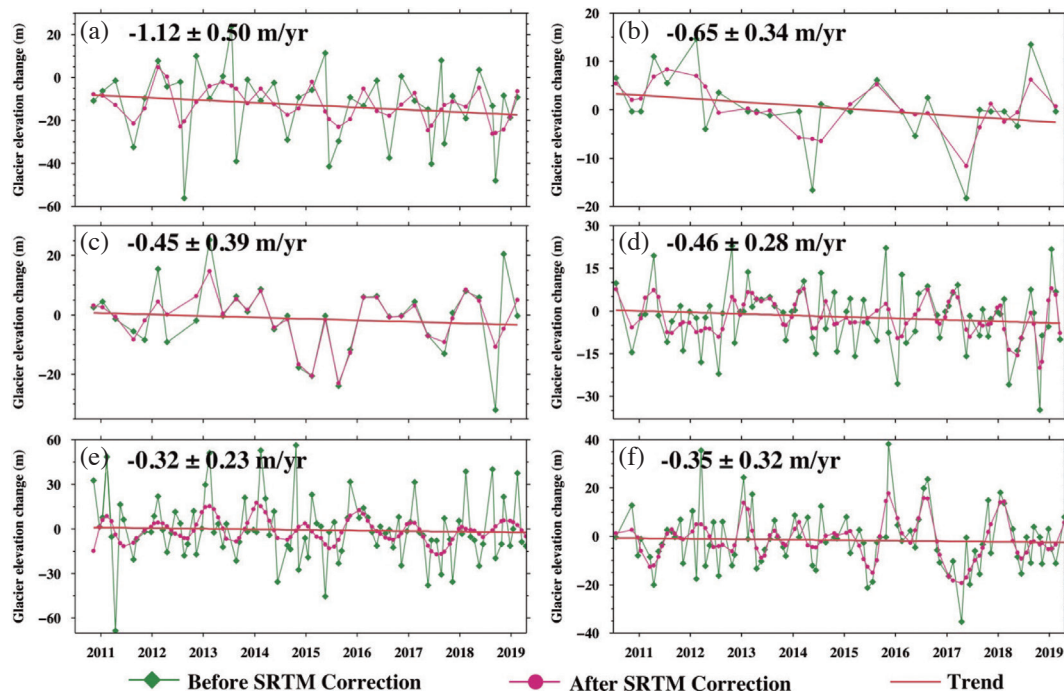
Fig. 9. Glacier elevation changes at sites A to F from Cryosat-2.
