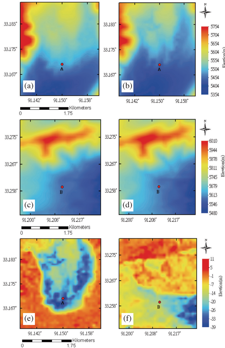
Fig. 11. Elevations at (a) site A from SRTM, (b) site A from TanDEM-X, (c) site B from SRTM, and (d) site B from TanDEM-X. Elevation differences at (e) site A, and (f) site B.
