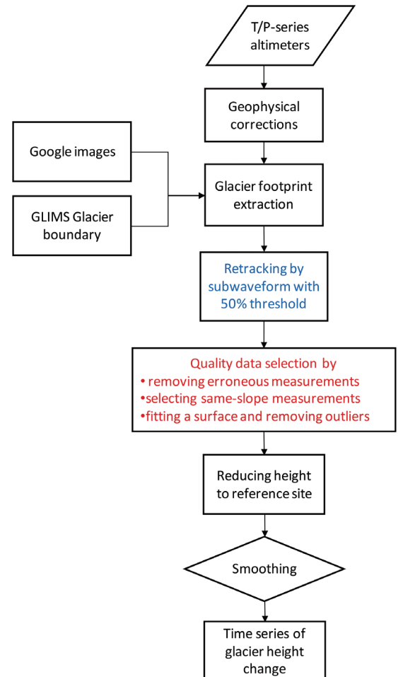
Fig. 4. Flowchart for constructing time series of glacier elevation changes from the T/P-Jason altimeters.
