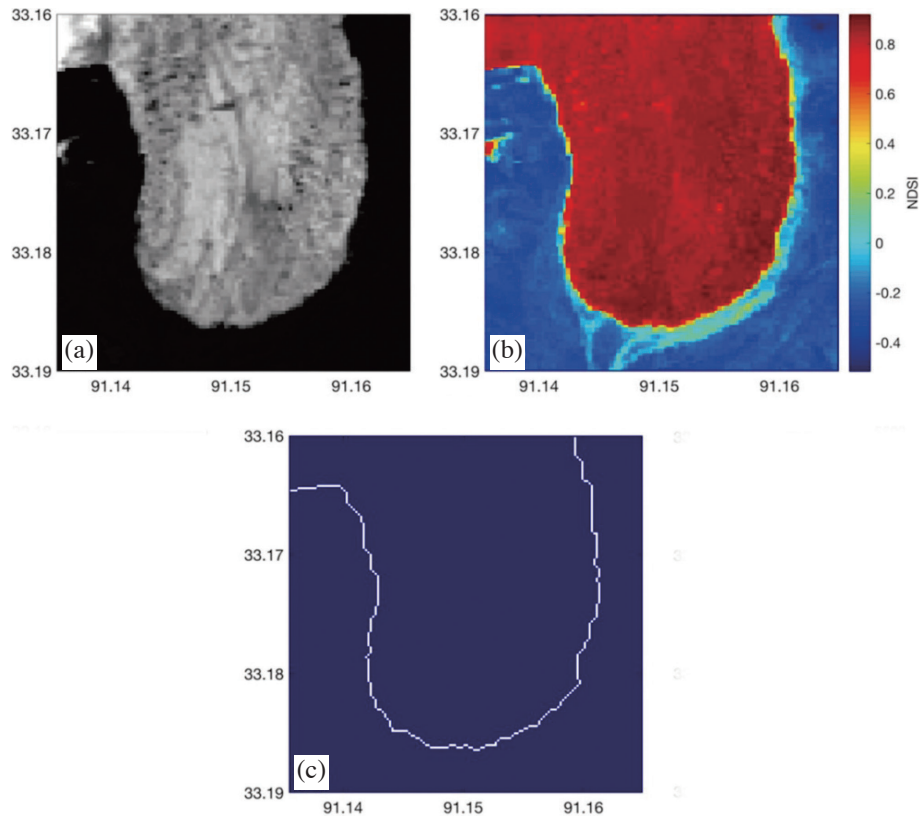
Fig. 7. Sample results for determining glacier area and edge around site A. (a) A cloud-free Landsat-5 image 1986. (b) NDSI values from this image [Eq. (13)]. (c) The glacier edge (white line) from NDSI using the threshold value NDSI \geq 0.4 (ice). This example shows that the glacier coverage near site A can be estimated with a Landsat image that is 35 years old (from 2020), demonstrating Landsat's capability to detect long-term glacier change.
