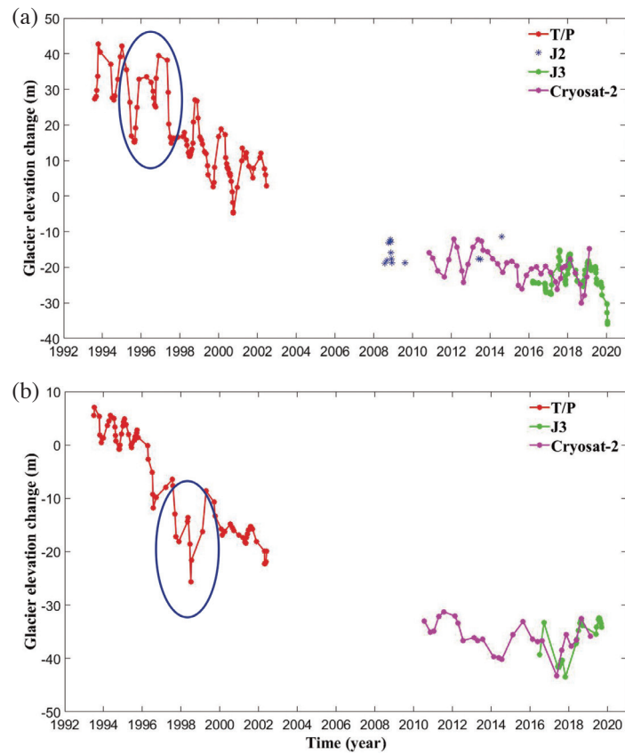
Fig. 8. Glacier elevation changes from the T/P-Jason and Cryosat-2 altimeters over 1993–2020 at site A (a), and site B (b). The blue ellipses highlight the elevation changes over 1997–1998 El Niño.
