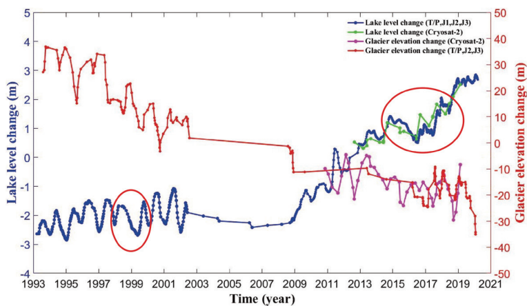
Fig. 13. Lake level changes over Chibuzhang Co and glacier elevation changes at site A from altimeters. The two red ellipses highlight the sudden drops in lake level after the 1997–1998 and 2014–2016 El Niño.
